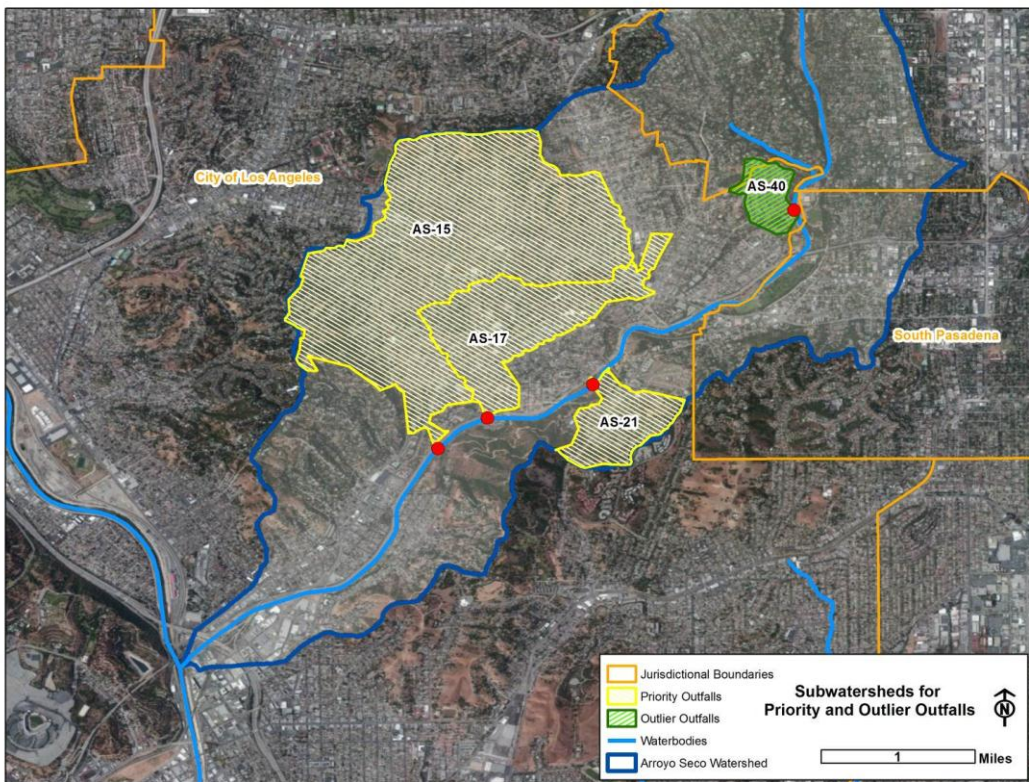
Figure 7-29. Drainage Areas for Preliminary Priority and Outlier Outfalls in City of LA Jurisdictional Area in Arroyo Seco Watershed
