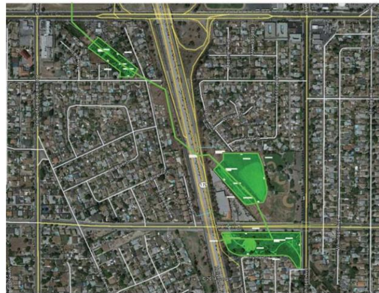
Proposed connection from Tujunga Spreading Grounds and modifications at Strathern Park, future site of a stormwater capture and infiltration project.
