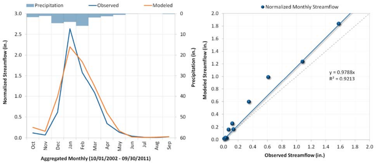
Figure A-3. Aggregated monthly hydrograph LACFCD F193-B, Santa Anita Wash At Longdem Avenue (10/1/2002 – 9/30/2011).
