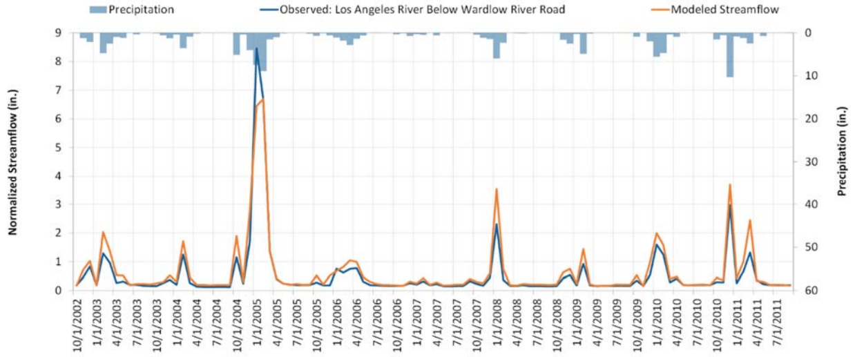
Figure A-12. Monthly hydrograph for LACFCD F318, Los Angeles River Below Wardlow River Road (10/1/2002 – 9/30/2011).
