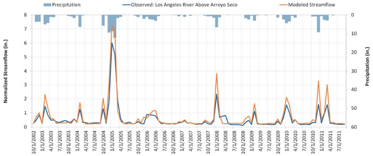
Figure A-16. Monthly hydrograph for LACFCD F57C, Los Angeles River Above Arroyo Seco (10/1/2002 – 9/30/2011).
