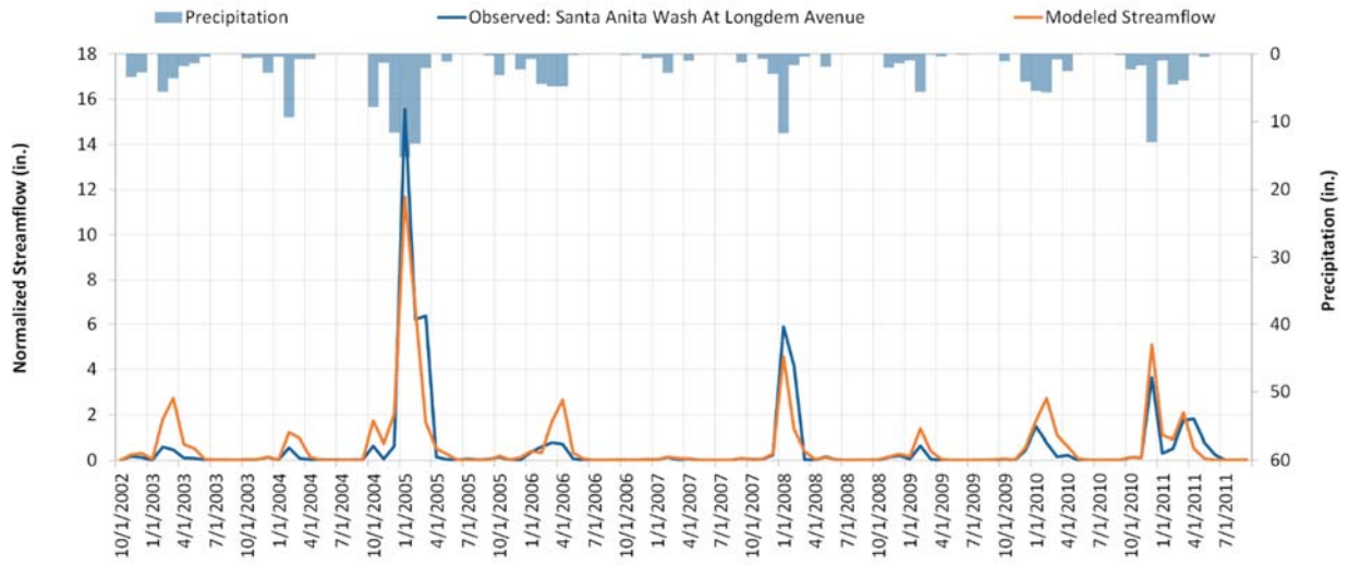
Figure A-2. Monthly hydrograph for LACFCD F193-B, Santa Anita Wash At Longdem Avenue (10/1/2002 – 9/30/2011).
