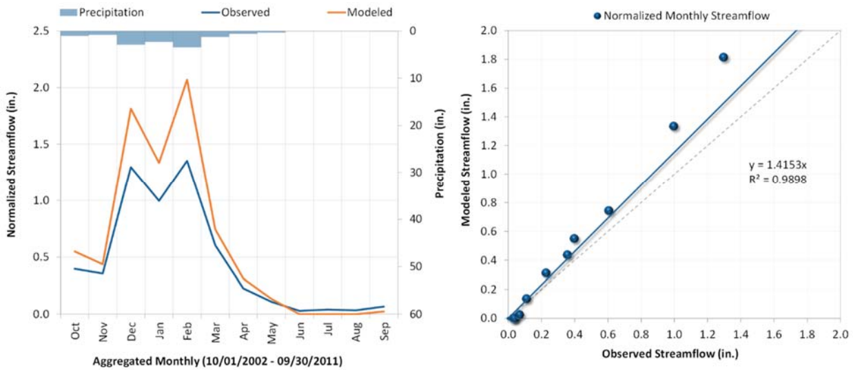
Figure A-21. Aggregated monthly hydrograph LACFCD F37B, Compton Creek Near Greenleaf Drive (10/1/2002 – 9/30/2011).
