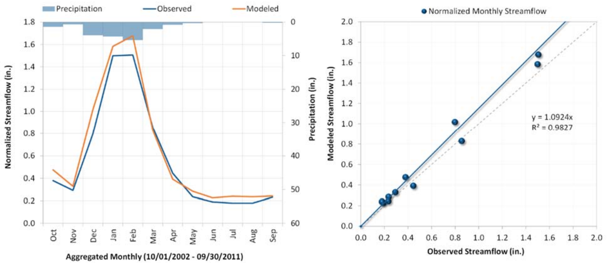
Figure A-17. Aggregated monthly hydrograph LACFCD F57C, Los Angeles River Above Arroyo Seco (10/1/2002 – 9/30/2011).
