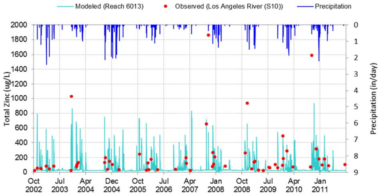
Figure A-25. Simulated vs. observed time series plots for Total Zinc at Los Angeles River mass emission station S10 (10/1/2002 through 9/30/2011).
