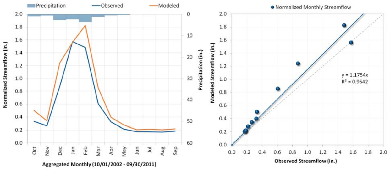
Figure A-13. Aggregated monthly hydrograph LACFCD F318, Los Angeles River Below Wardlow River Road (10/1/2002 – 9/30/2011).
