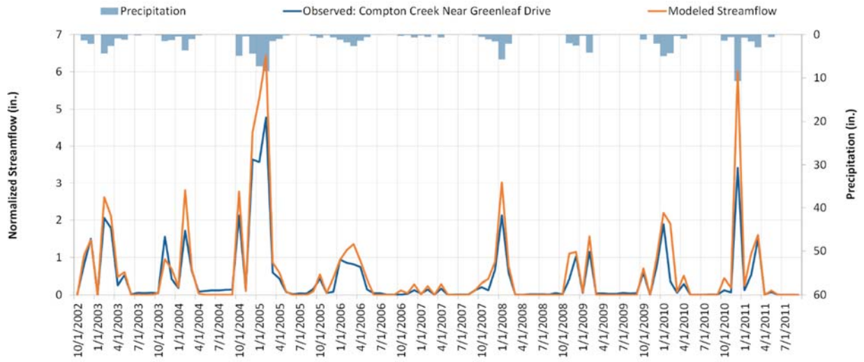
Figure A-20. Monthly hydrograph for LACFCD F37B, Compton Creek Near Greenleaf Drive (10/1/2002 – 9/30/2011).
