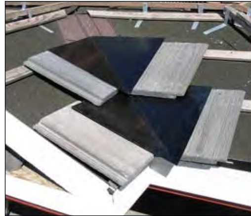
Figure 2. Special valley flashing to avoid debris accumulation between and below tiles (photograph courtesy of MonierLifetile).
