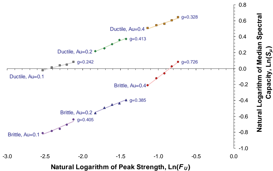
Figure E-22 Plot showing effect of variation in peak strength, F_U , on median spectral capacity, S_{\mu} for various configurations of material form and upper-story strength ratio, A_U . The median spectral capacity is determined using the Onset of Strength Loss (OSL) set of drift criteria. Ductile materials are those with high-displacement capacity ( C_D=1.0 ). Brittle materials are those with low-displacement capacity ( C_D=0.0 ). The value, g , is the gradient (slope) quantifying the effect of the variation.
