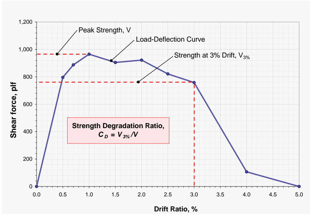
Figure 4-15 Load-drift curve depicting determination of strength degradation ratio, C_D .
