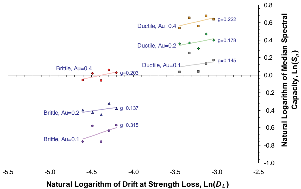
Figure E-23 Plot showing effect of variation in drift at strength loss, D_L , on median spectral capacity, S_{\mu} , for various configurations of material form and upper-story strength ratio, A_U . The median spectral capacity is determined using the Onset of Strength Loss (OSL) set of drift criteria. Ductile materials are those with high-displacement capacity ( C_D=1.0 ). Brittle materials are those with low-displacement capacity ( C_D=0.0 ). The value, g , is the gradient (slope) quantifying the effect of the variation.
