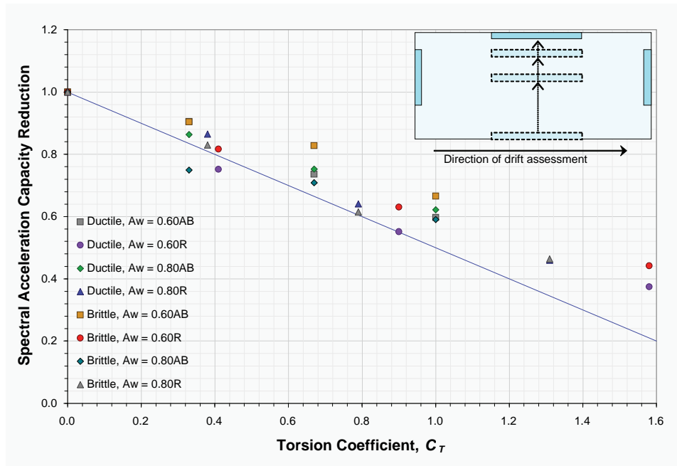
Figure E-38 Plots of spectral acceleration capacity reduction versus torsion coefficient, C_T , for the Onset of Strength Loss set of drift criteria, considering the longitudinal direction for various values of weak-story ratio, A_w . “AB” indicates unretrofitted model; “R” indicates model with optimal retrofit.
