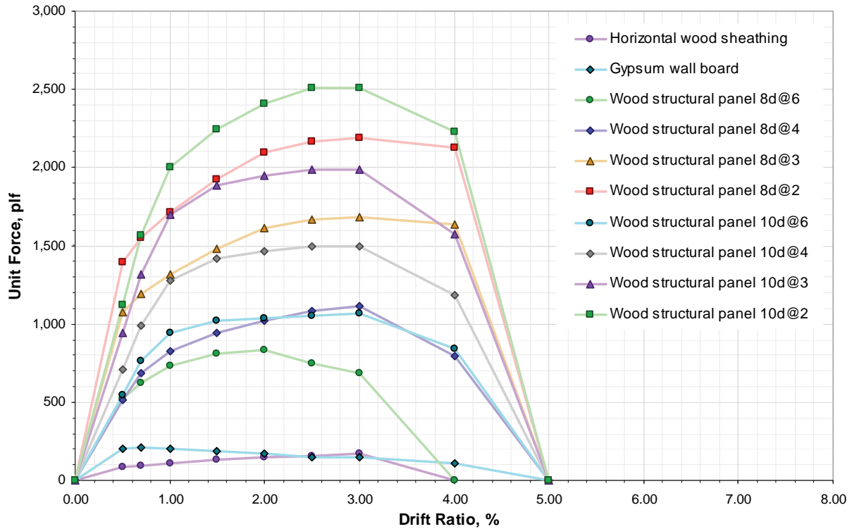
Figure 4-1 Unit load-drift curves for sheathing materials with high-displacement capacity. Wall-panel nailing notation: nail size (e.g., 8d) @ distance between center of nails in inches.
