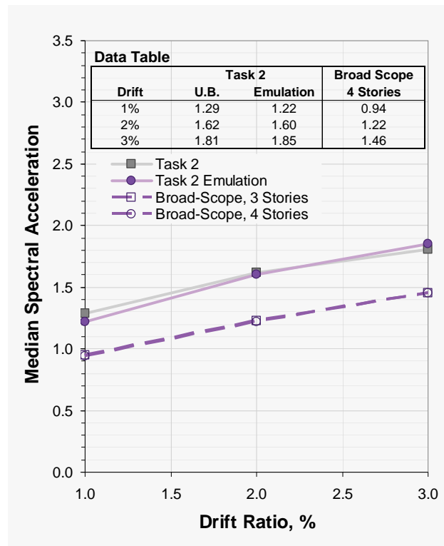
Figure F-11 Comparison of analysis results for the building with retrofit strength of V_y/V_2 of 0.2 for Task 2 and emulation of Task 2 and V_y/V_2 of 0.2 for the Broad-Scope Analysis .
