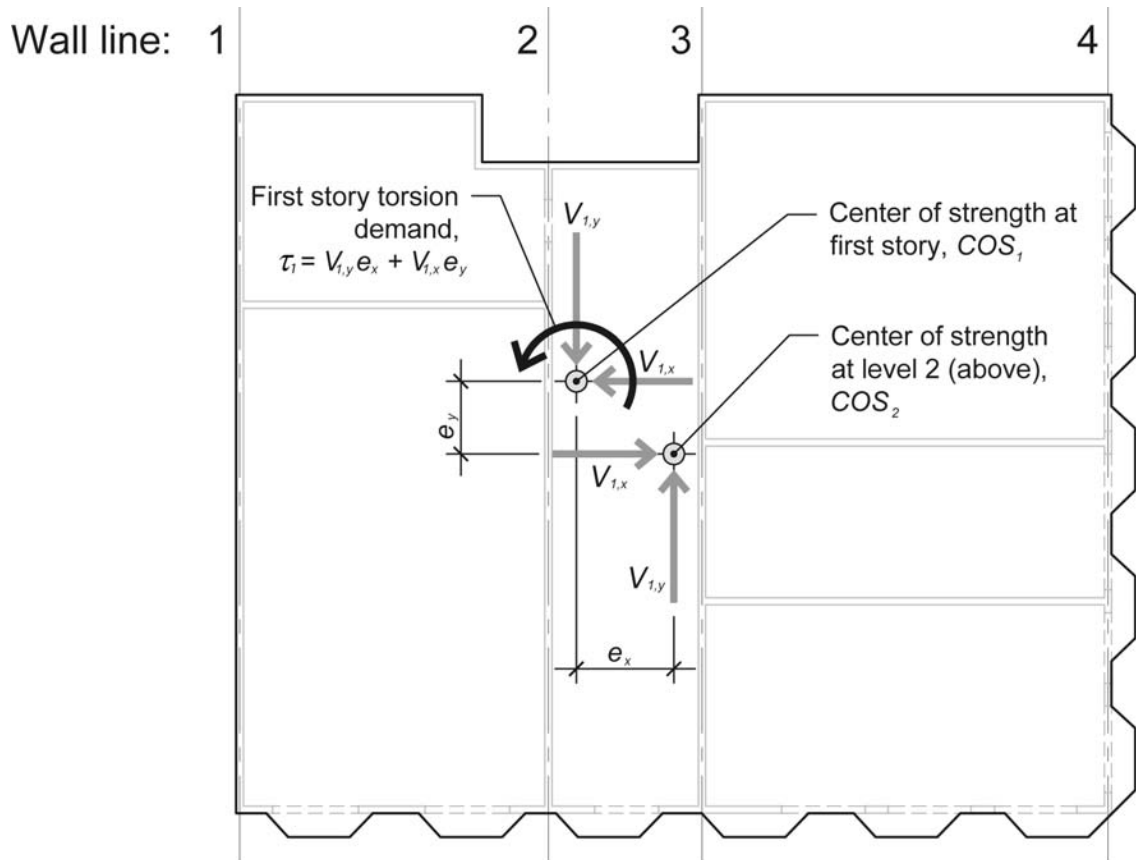
Figure 4-14 Wall-plan schematic depicting how the torsional demand on the first story is calculated.
