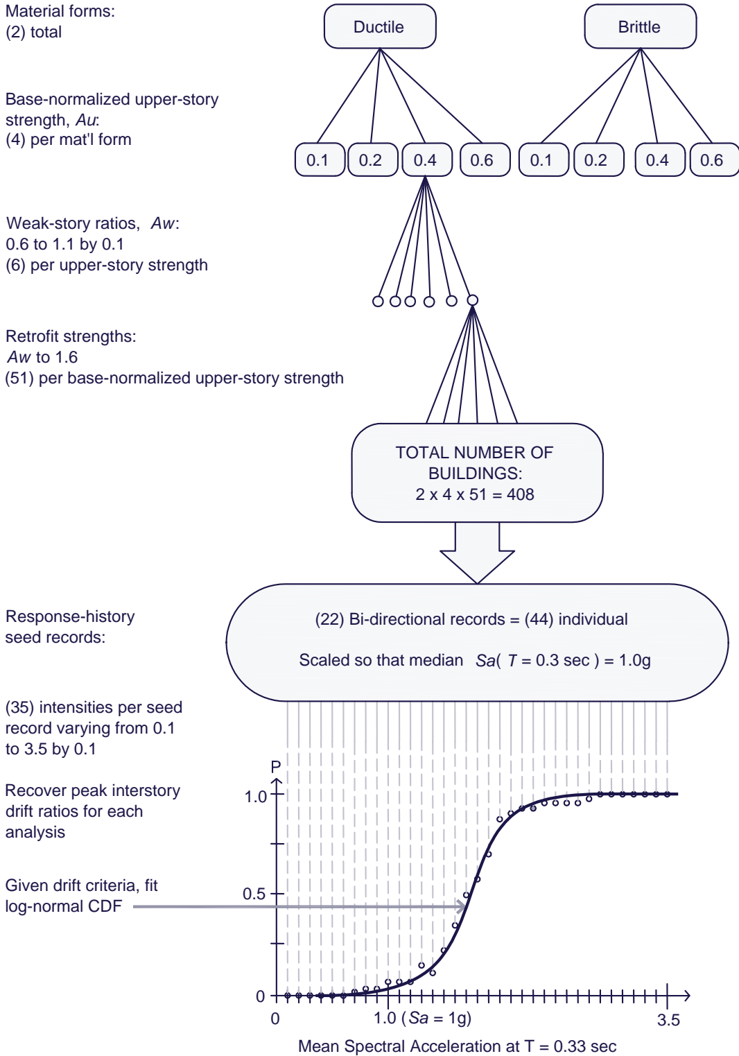
Figure E-12 Flow chart used in translational analyses to optimize retrofit. Ductile materials are those with high-displacement capacity; brittle materials are those with low-displacement capacity. CDF = Cumulative Distribution Function. S_a = spectral acceleration. T = period of oscillation. P = probability of not being exceeded.
