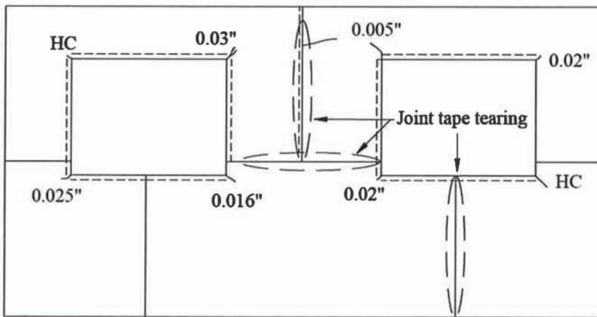
Figure D-24 Crack maps for gypsum wallboard sheathing at 0.7% drift for (top) Wall 1 and (bottom) Wall 2. Crack width and length increased. Nail pops increased. Crushing of the gypsum core occurred at window corners in compression. Tearing of the joint tape occurred, leading to wall board panels rotating individually (from Arnold, Uang and Filiatrault, 2003).
