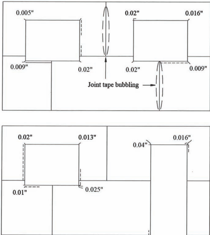
Figure D-23 Crack maps for gypsum wallboard sheathing at 0.4% drift for (top) Wall 1 and (bottom) Wall 2. Cracking at corners and edges of windows increased. Joint tape bubbling and nail popping started to occur (from Arnold, Uang and Filiatrault, 2003).
