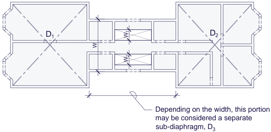
Figure 2-11 Floor plan schematic showing diaphragm openings that must be limited in size to satisfy eligibility requirements. D denotes diaphragm.
