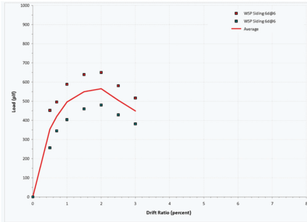
Figure D-7 Load-drift data for wood structural panel siding (5/16" and 3/8" thickness). Additional information on testing procedures for each data source is provided in Table D-7.
